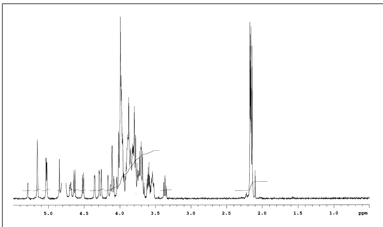
Figure 1 : 500 MHz ^1\text{H-NMR} of HYBRID Glycan (Cat. No.CN-HYBRID-20U, Lot No. A15L-03)
