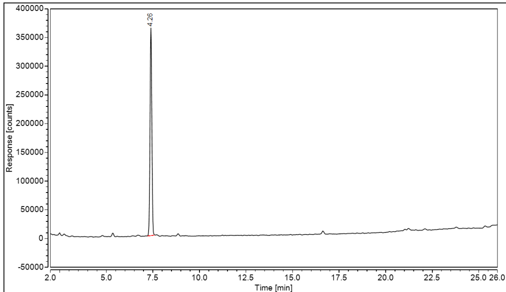
Figure 1: HILIC HPLC profile of two 2AB labelled GLIP-GM1-01 glycans (Batch: C01G-01) released using LZ-CER-HM-KIT (Batch: C01G-04)
