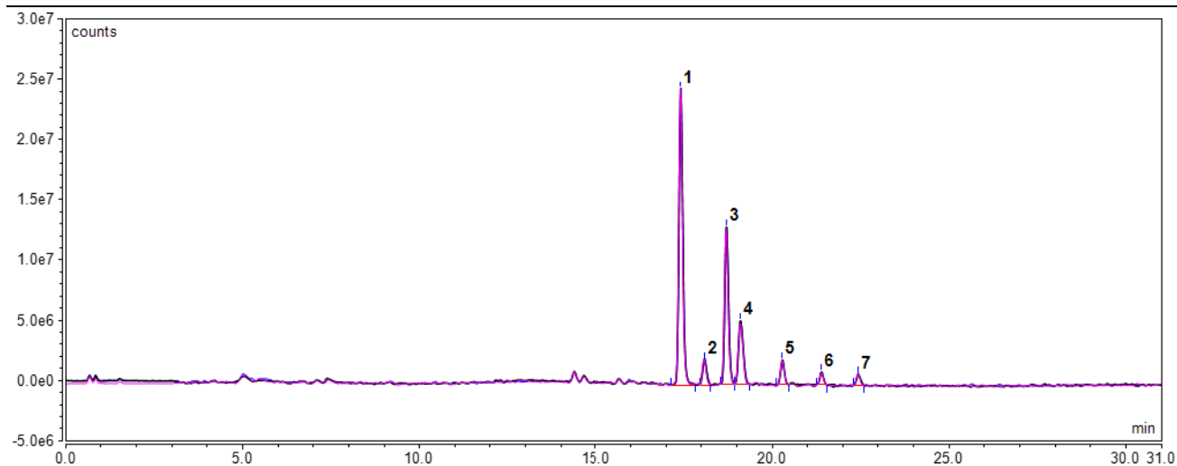
Figure 1: HILIC HPLC profile of three tryptic IgG-1 glycopeptide samples (10ug weight of protein before digest) labeled using LT-VTAG-24 (Batch B547-04 )
