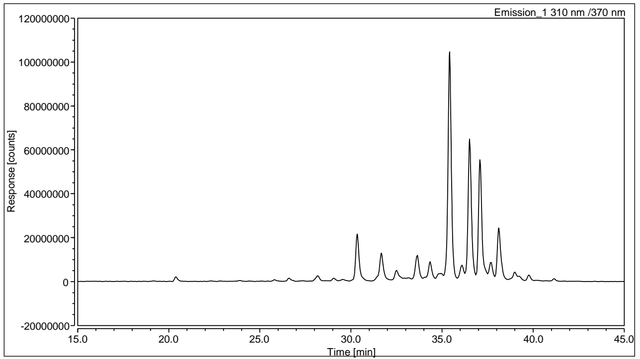
Figure 2. BEH Glycan column UHPLC profile of procainamide labeled N-glycans released from bovine fetuin by PNGase F digestion
