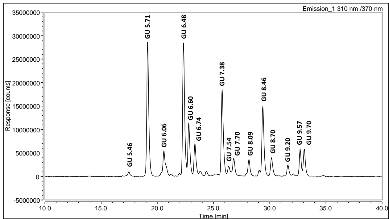
Figure 1. BEH Glycan column UHPLC profile of procainamide labeled N-glycans released from human IgG by PNGase F digestion
