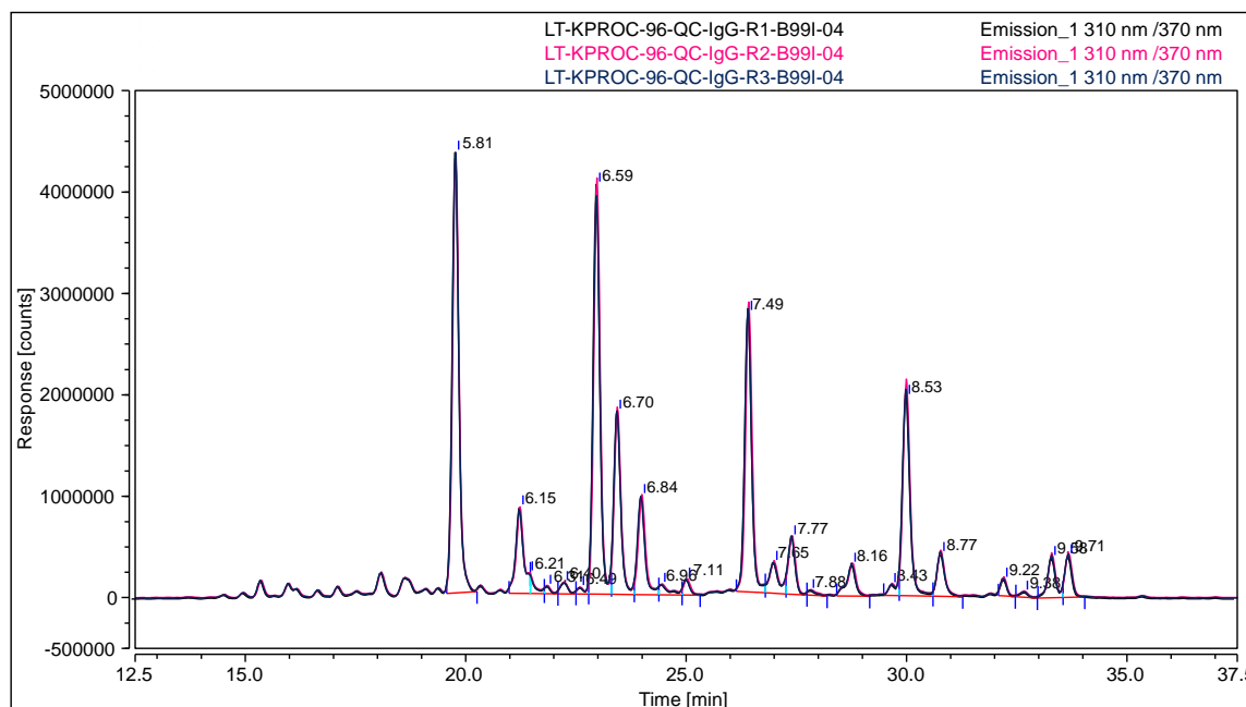
Figure 1: BEH Glycan column UHPLC profile of procainamide labeled N-glycans released from human IgG by hydrazinolysis.
