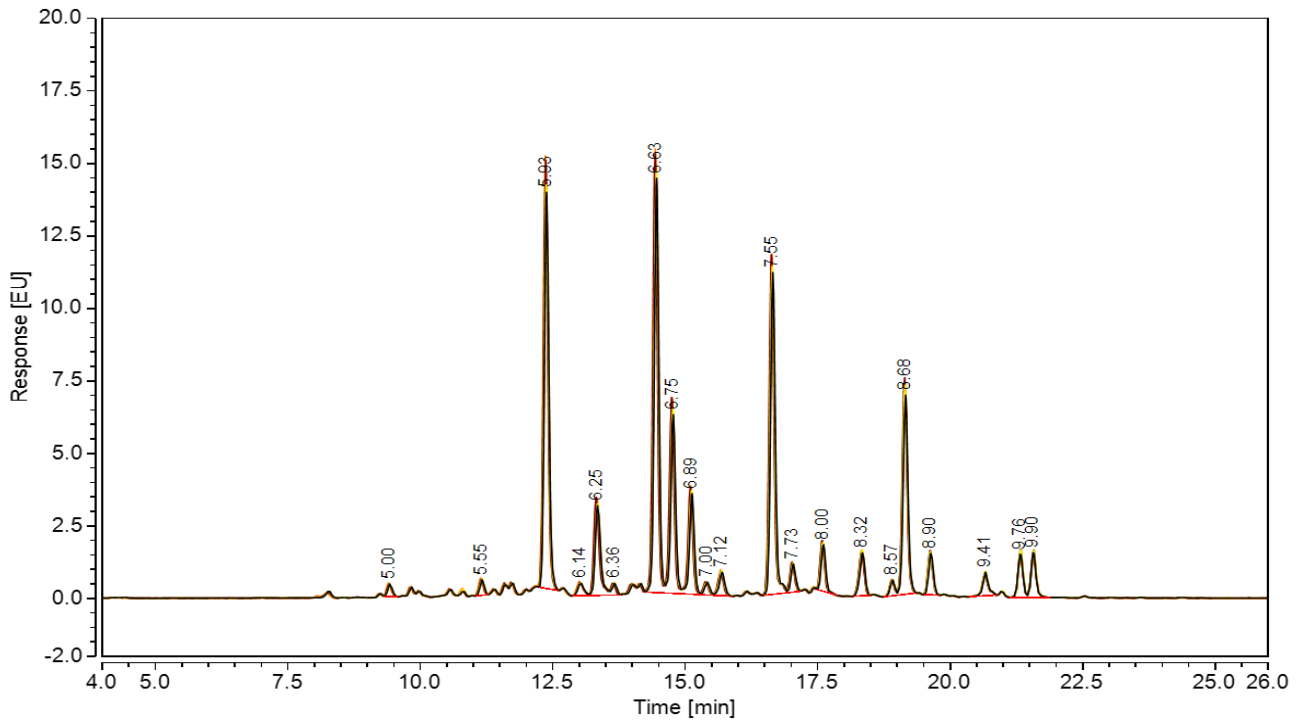
Figure 1: HILIC HPLC profile of three Human-IgG glycan samples (Cat. #: CLIBN-IGG-5U (Batch B9BM-01) labelled using LT-KAB-VP24 (Batch C034-03)
