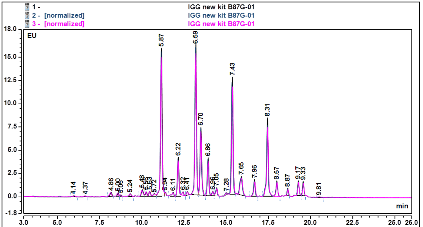
Figure 1: HILIC HPLC profile of three Human-IgG glycan samples (Cat. #: CLIBN-IGG-5U Batch B78A-01) labeled using LT-KAB-VP24 (Batch B87G-01)
