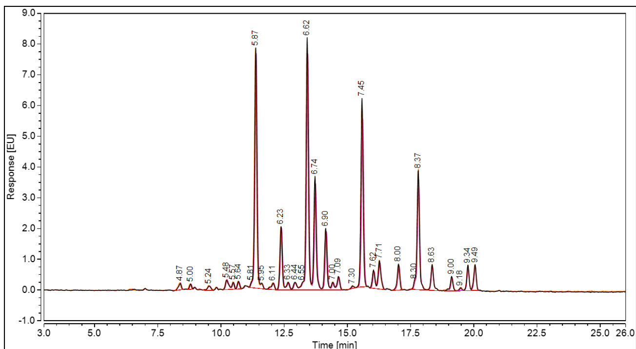
Figure 1: HILIC HPLC profile of three Human-IgG glycan samples (Cat. #: CLIBN-IGG-5U Batch B78A-01) labeled using LT-KAB-VP24 (Batch B85I-02)
