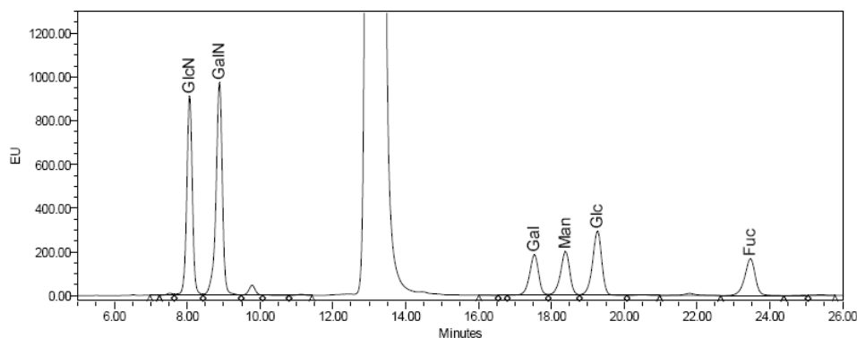
Figure 1: LudgerSep-R2 profile of CM-Mono-Mix-10 -2AA labelled - monosaccharide gradient. Date of Analysis – 17 Mar 2020
