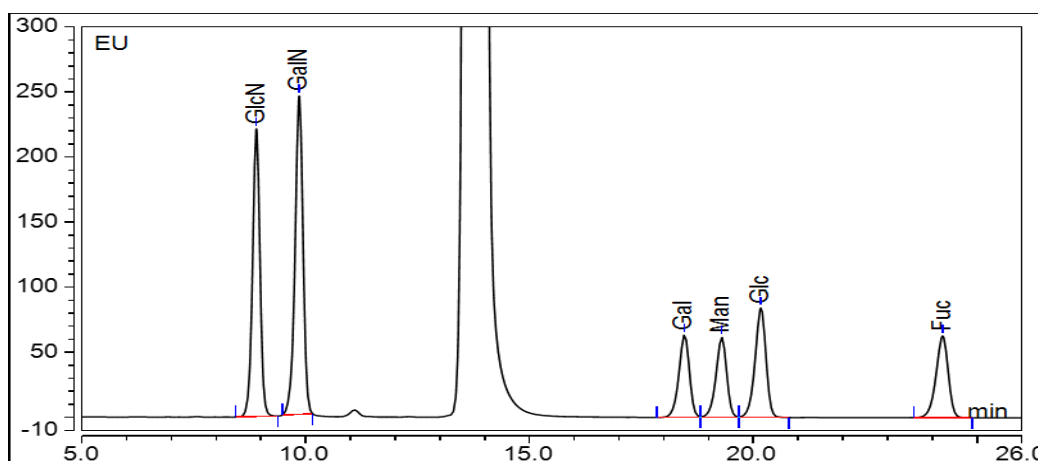
Figure 1: LudgerSep-R2 profile of CM-Mono-Mix-10 -2AA labelled - monosaccharide gradient. Date of Analysis – 07 Feb 2020
