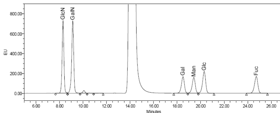
Figure 1: LudgerSep-R2 profile of CM-Mono-Mix-10 -2AA labelled - monosaccharide gradient. Date of Analysis – 28 Sep 2018
