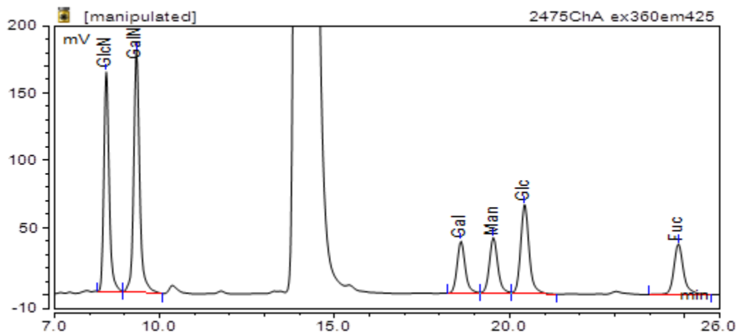
Figure 1: LudgerSep-R2 profile of CM-Mono-Mix-10 -2AA labelled - monosaccharide gradient. Date of Analysis – 05 June 2017.
