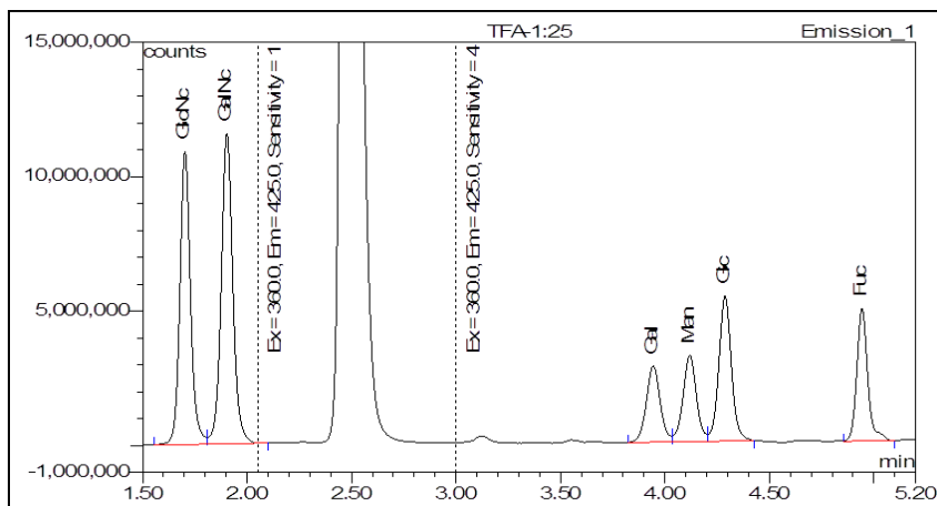
Figure 1. LudgerSep-uR2 profile of CM-Mono-Mix-10 -2AA labelled - monosaccharide gradient. Date of Analysis – 10 July 2014.
