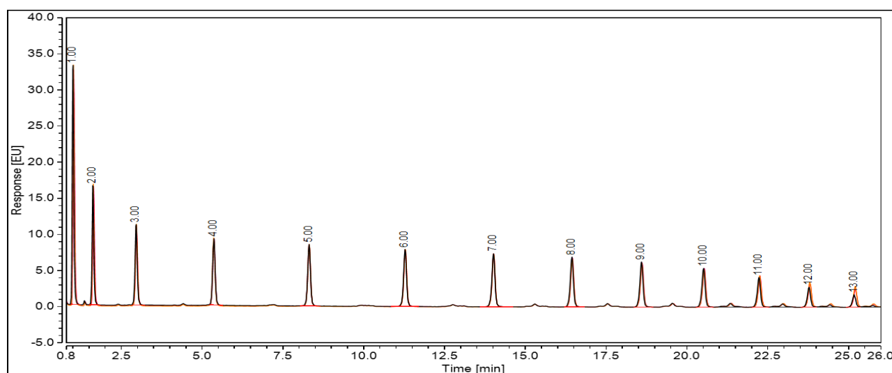
Figure 1: CAB-GHP-30 - N-glycan gradient – three replicates overlaid. Samples run 05 June 2018
