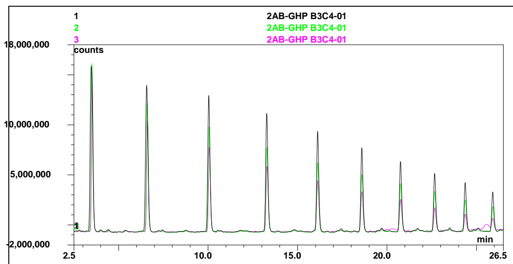
CAB-GHP-30 - N-glycan gradient – three replicates overlaid. Samples run Jul 2014.
