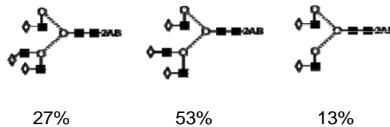
Figure 4. Relative amount of each core type of N-glycan, after removal of sialic acids, from a similar batch of GCP-FET.
