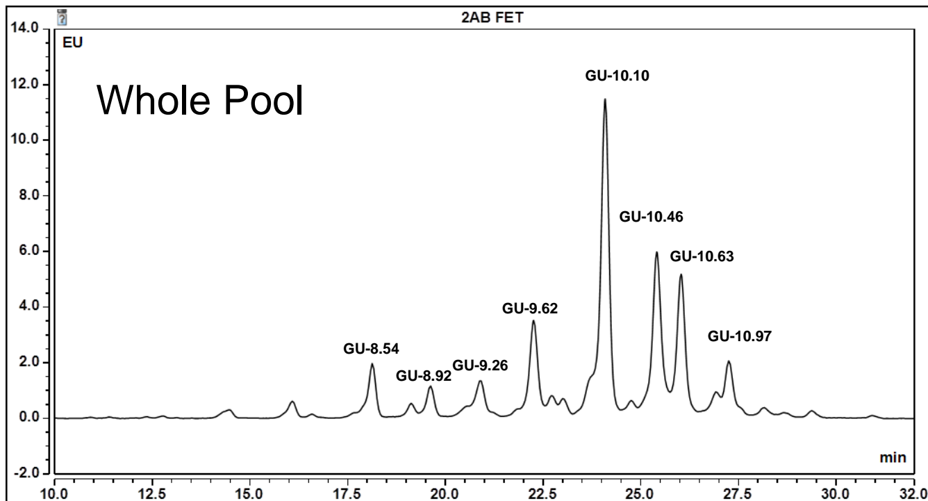
Figure 1. HILIC HPLC profile of 2-AB labeled Fetuin N-glycans, released by PNGase F from GCP-FET-50U batch B88L-01 run on Waters BEH Glycan column.
