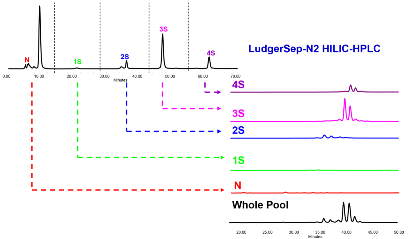
Figure 2. LudgerSep-C3 profile and subsequent LudgerSepN2 analysis of bovine fetuin PNGaseF released N-glycans from a similar batch of GCP-FET.
