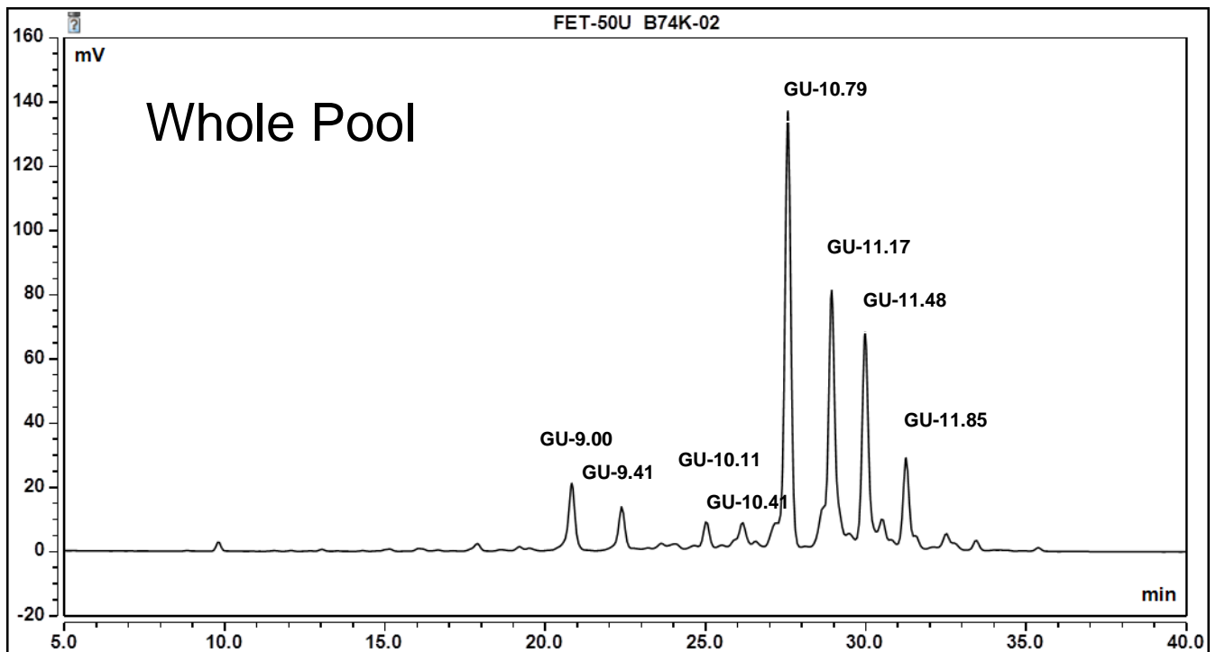
Figure 1: HILIC HPLC profile of 2-AB labelled Fetuin N-glycans, released by PNGase F from GCP-FET-50U batch B74K-02 run on Waters BEH Glycan column.
