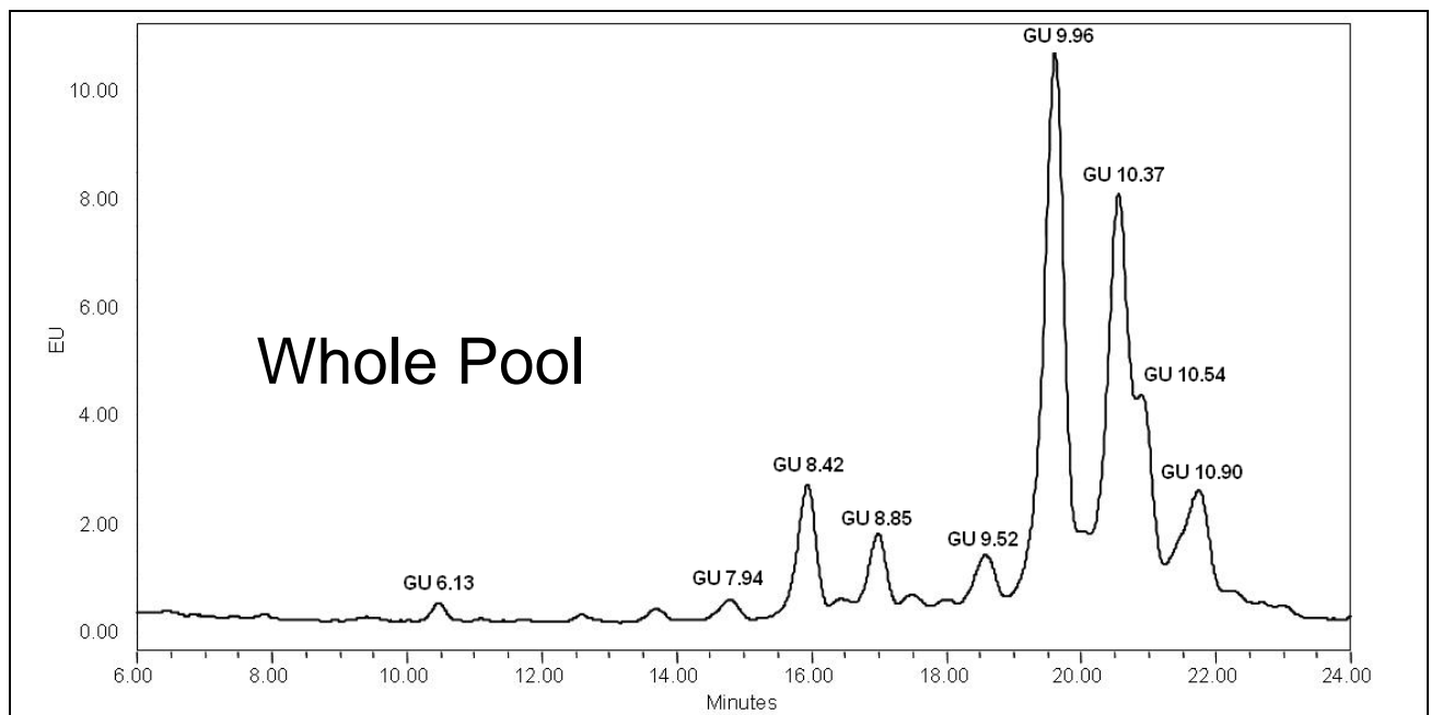
Figure 1: LudgerSepN2 (Cat. #: LS-N2-4.6x150) HPLC profile of 2-AB labelled Fetuin N-glycans, released by PNGase F from GCP-FET-50U batch B144-02.
