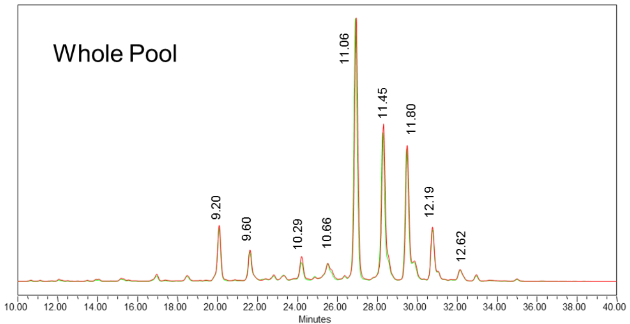
Figure 1: HILIC HPLC profile of 2-AB labelled Fetuin N-glycans, released by PNGase F from GCP-FET-250U batch B54U-02 run on Waters BEH Glycan column.
