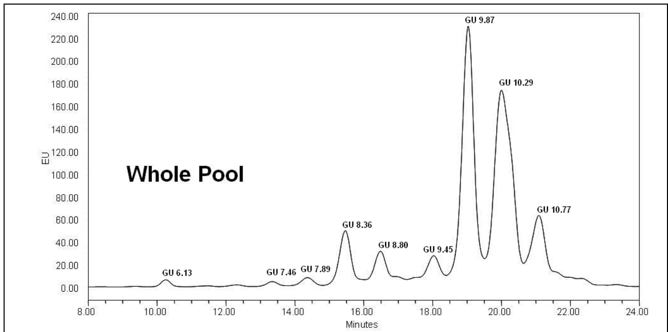
Figure 1: LudgerSepN2 (Cat. #: LS-N2-4.6x150) HPLC profile of 2-AB labelled Fetuin N-glycans, released by PNGase F from GCP-FET-250U batch B06L-03.
