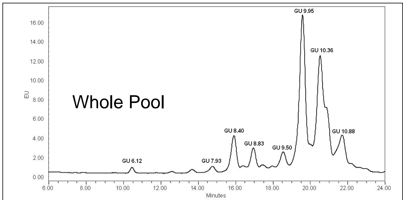
Figure 1: LudgerSepN2 (Cat. #: LS-N2-4.6x150) HPLC profile of 2-AB labelled Fetuin N-glycans, released by PNGase F from GCP-FET-100U batch B148-01.
