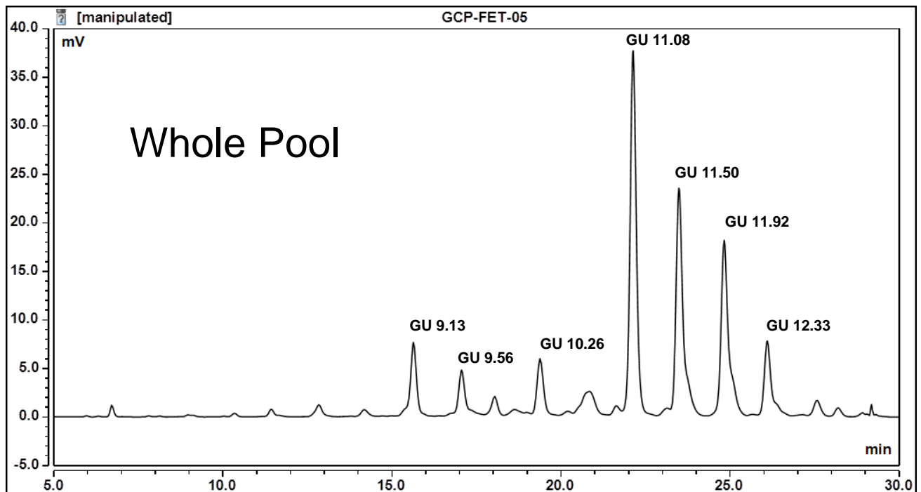
Figure 1: Waters BEH column HPLC profile of 2-AB labelled Fetuin N-glycans, released by PNGase F from GCP-FET-05 batch B1B2-04.
