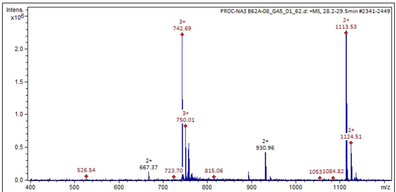
Figure 2: Positive ion mass spec analysis of labelled Glycan Sample. Main peak at m/z 1113.5 conforms to expected [M+H]^{2+} mass (peak at 742.7 conforms to [M+H]^{3+} mass). No significant unlabelled glycan peak present. (Cat. #: CPROC-NA3-01, Batch B62A-08).
