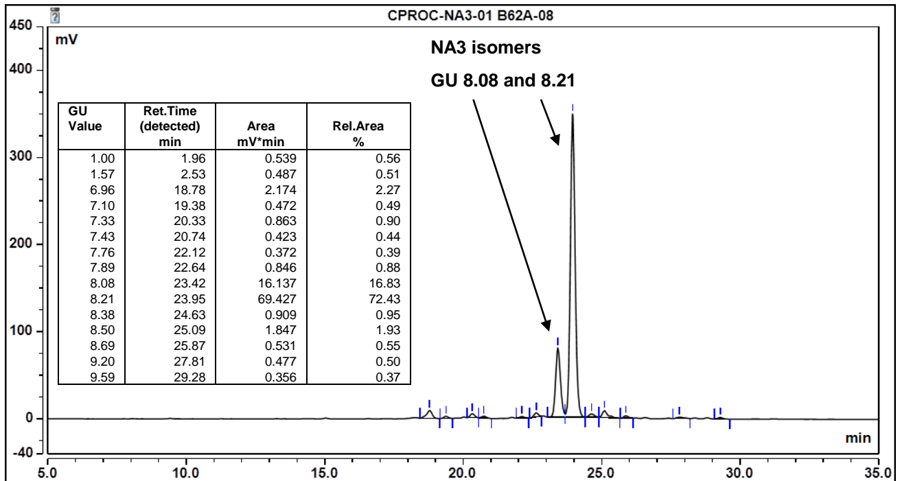
Figure 1: HILIC HPLC profile of Procainamide labelled NA3 glycan (see method conditions below) (Cat. #: CPROC-NA3-01, Batch B62A-08).
