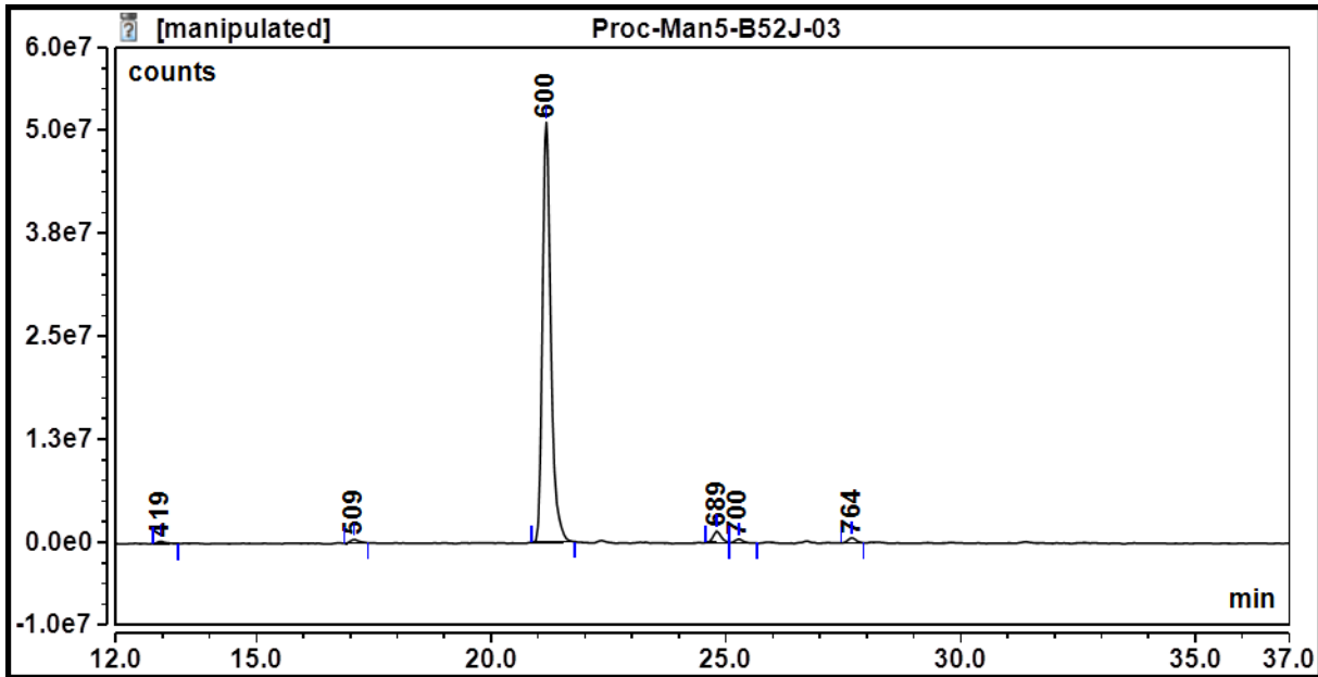
Figure 1: HILIC HPLC profile of Procainamide labelled Man5 glycan (see method conditions below) (Cat. #: CPROC-MAN5-01, Batch B52J-03 ).
