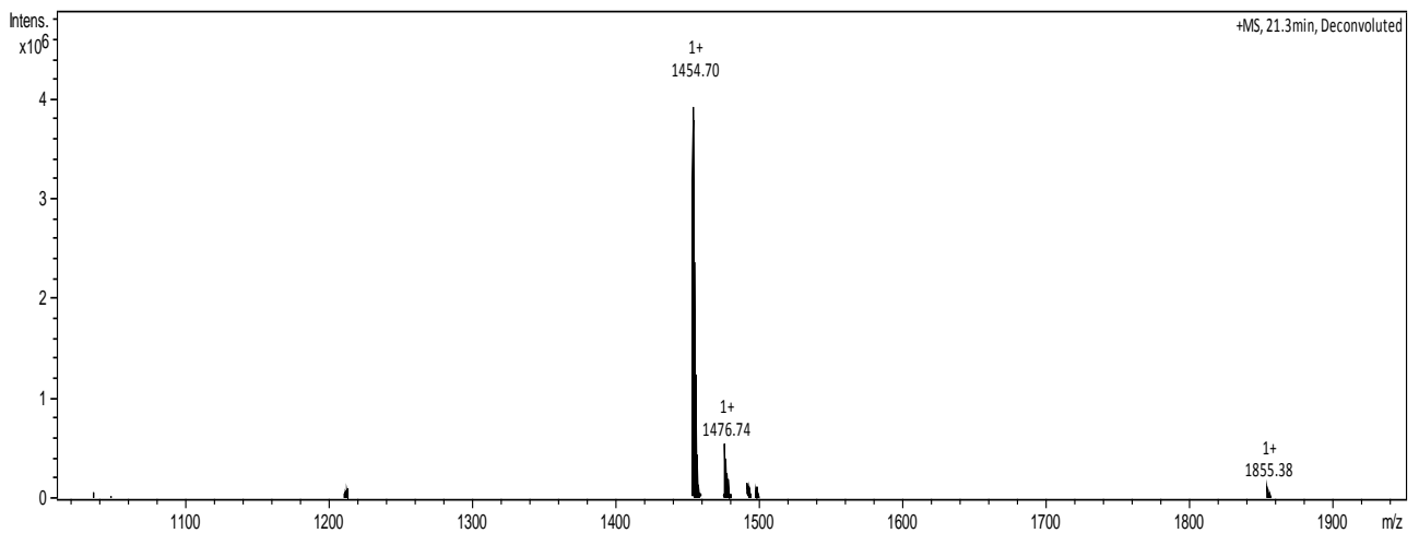
Figure 2: Positive ion mass spec analysis of labelled Glycan Sample. Main peak at m/z 1454.73 conforms to expected [M+H]^+ mass. No significant unlabelled glycan peak present. (Cat. #: CPROC-MAN5-01, Batch B52J-03).
