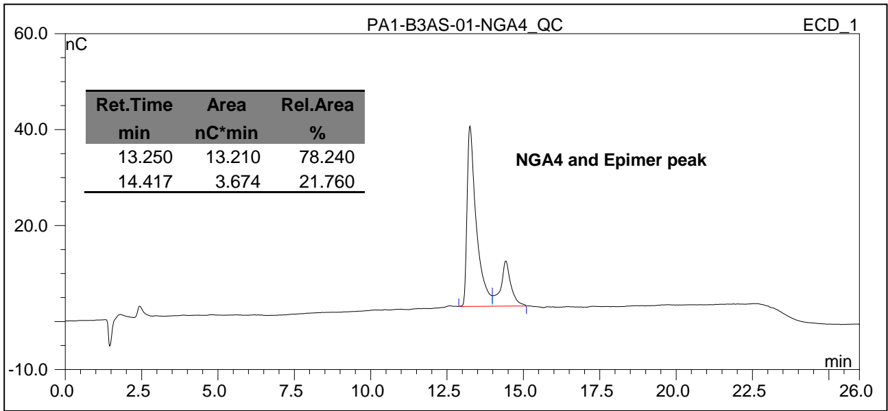
Figure 1: HPAE-PAD HPLC Profile of NGA4 Glycan (CN-NGA4-10U, Batch A652-03).
