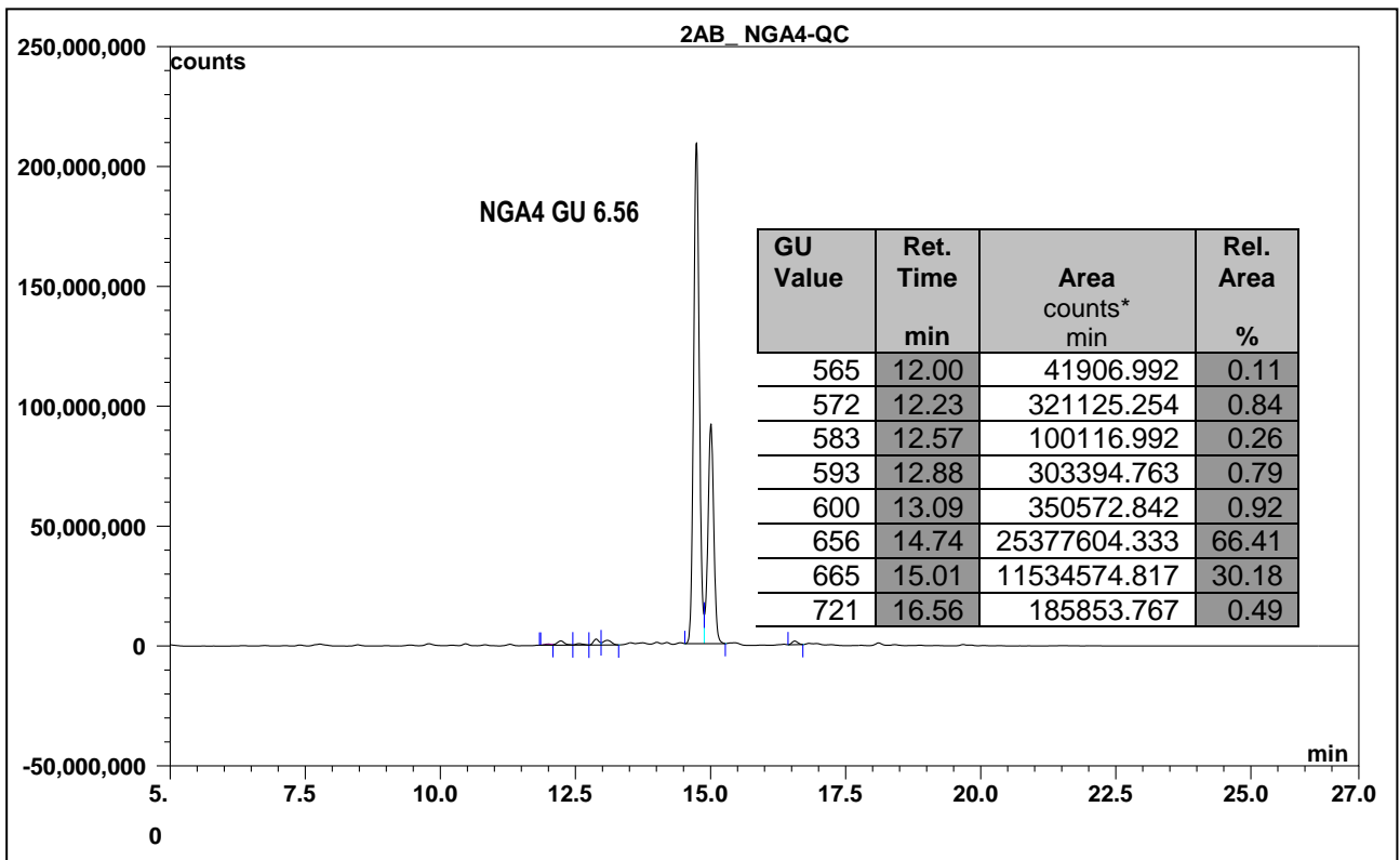
Figure2: BEH Glycan column chromatogram of 2AB labelled NGA4 glycan (CN-NGA4-10U, Batch A652-03).
