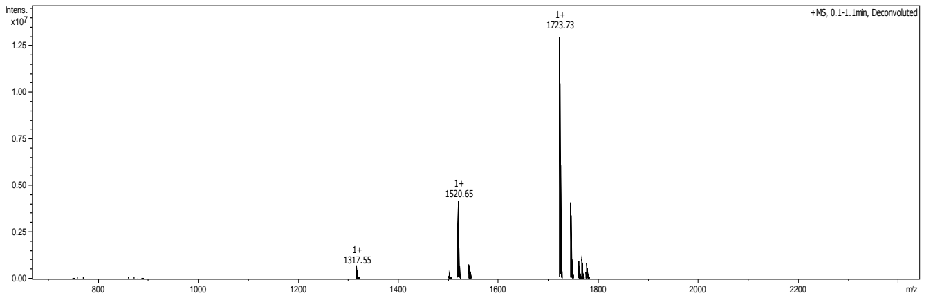
Figure 3: Positive ion mass spectrum of NGA4 glycan (CN-NGA4-10U, Batch A652-03). Theoretical mass 1724 Da [M+Na]^+ .
