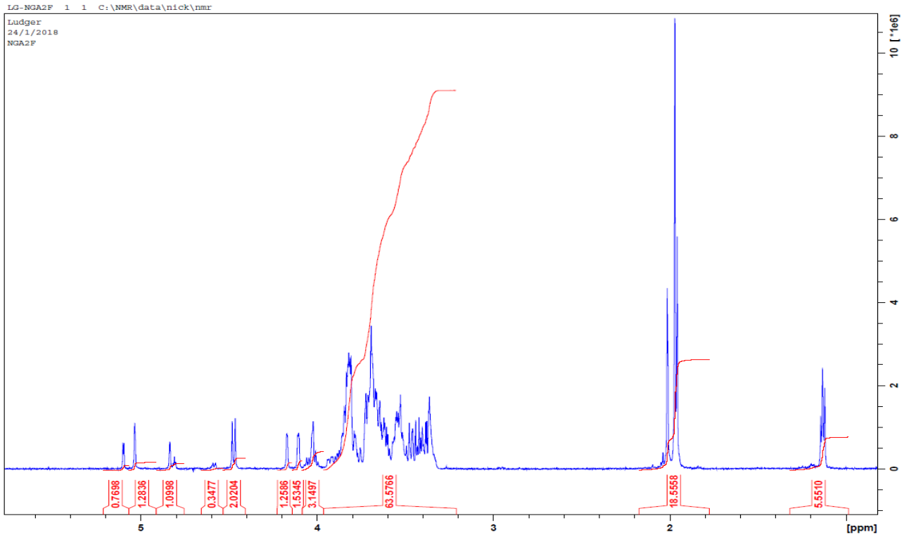
Figure 3: 500MHz ^1\text{H-NMR} of NGA2F glycan BULK (CN-NGA2F-BULK, Batch B81T-03)
