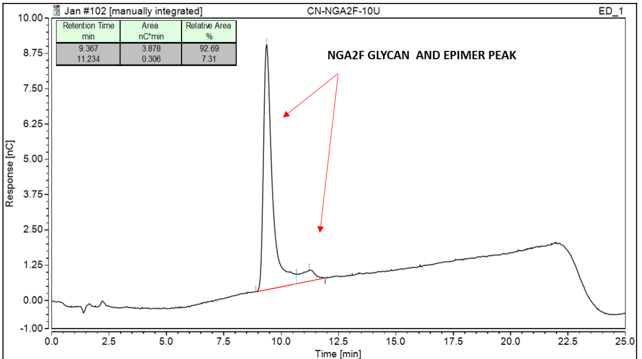
Figure 2: HPAE-PAD HPLC Profile of NGA2F (CN-NGA2F-10U, Batch B827-05)
