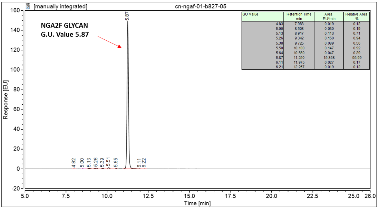
Figure 1: HILIC column UPLC chromatogram of 2AB labeled NGA2F glycan (CN-NGA2F-10U, Batch B827-05)
