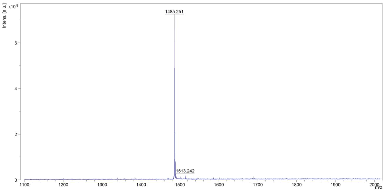
Figure 4: Positive ion mass spectrum of permethylated NGA2F glycan (CN-NGA2F-10U, Batch B827-05). Theoretical mass 1485.2 Da [\text{M}+\text{Na}]^+
