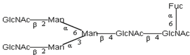
Text Notation
