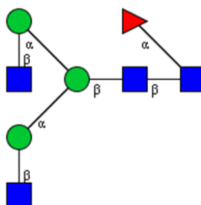
CFG Notation
