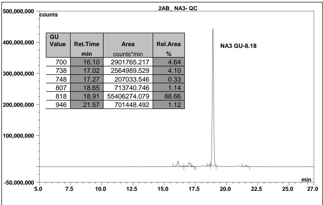
Figure 2: BEH Glycan column chromatogram of 2AB labelled NA3 glycan (CN-NA3-10U, Batch A68T-03).
