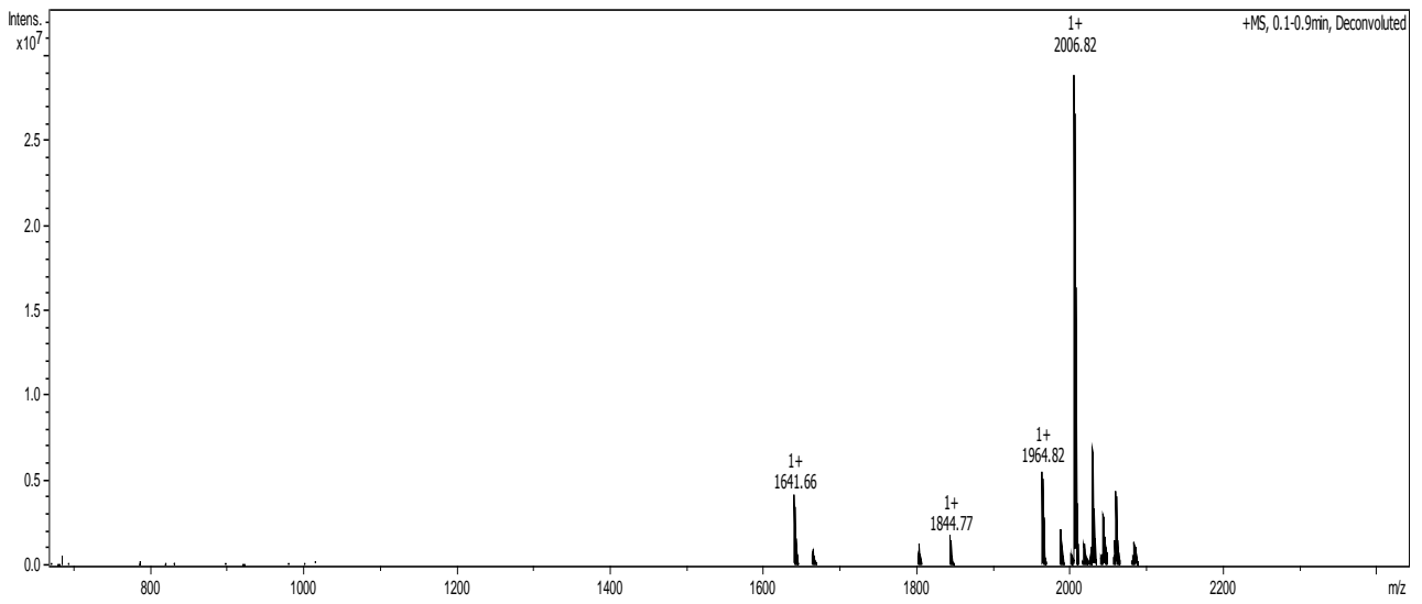
Figure 3: Positive ion mass spectrum of NA3 glycan (CN-NA3-10U, Batch A68T-03). Theoretical mass 2007 Da [M+Na]^+ .
