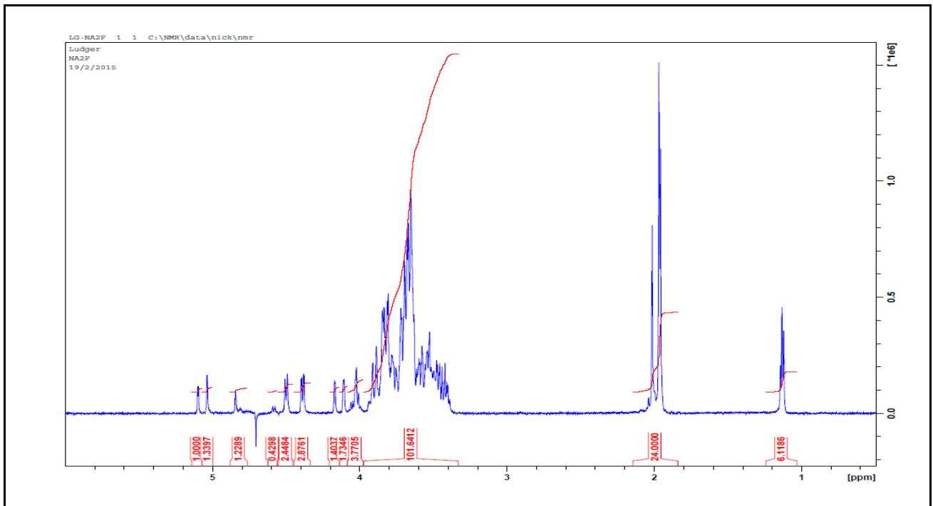
Figure 3: 500MHz 1 H-NMR of NA2F glycan BULK (CN-NA2F-BULK, Batch B533-02).
