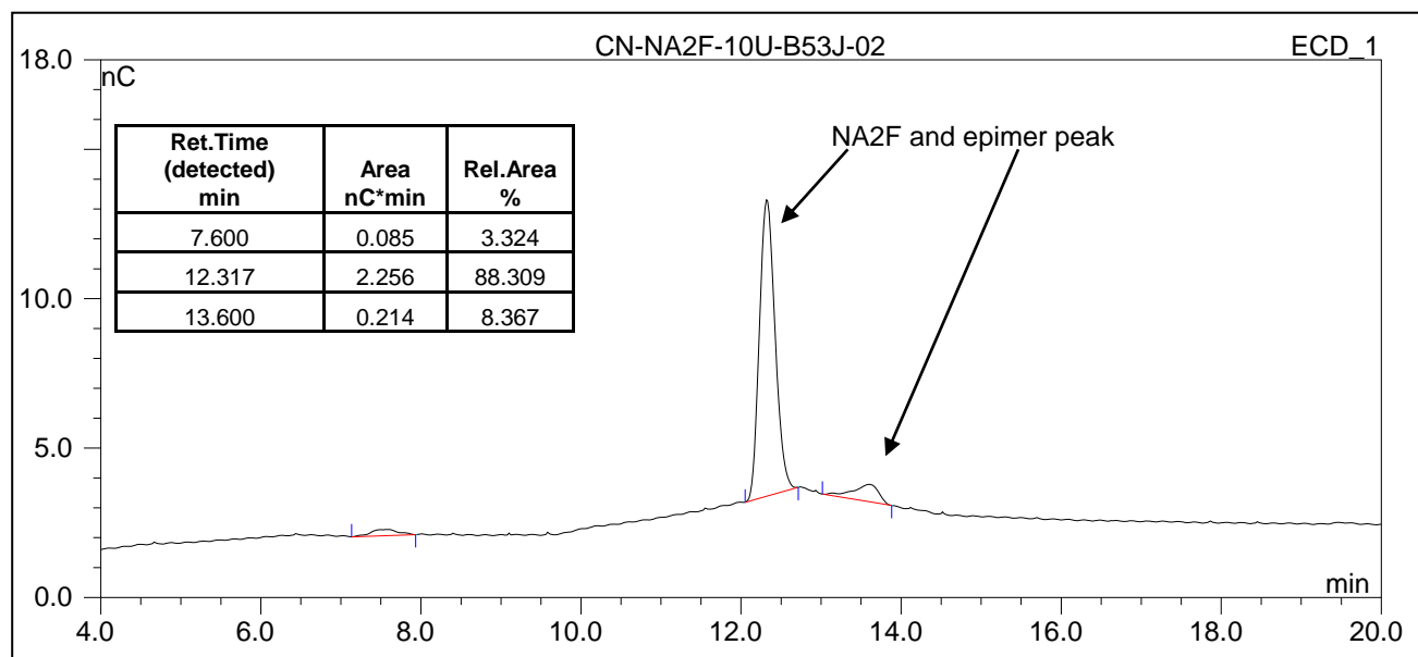
Figure 2: HPAE-PAD HPLC Profile of NA2F (CN-NA2F-10U, Batch B53J-02).
