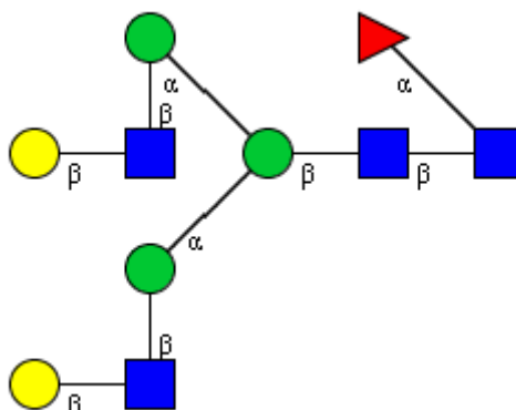
CFG Notation
