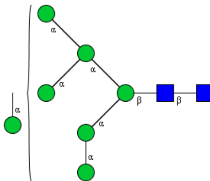
CFG Notation
