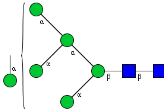
CFG Notation
