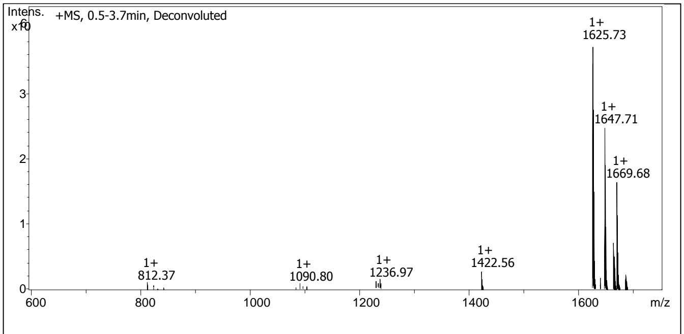
Figure 4: Positive ion mass spectrum of permethylated FA2G1 glycan (CN-FA2G1-10U, Batch B3B8-01). Theoretical mass 1625.6 Da [M+H]^+ .
