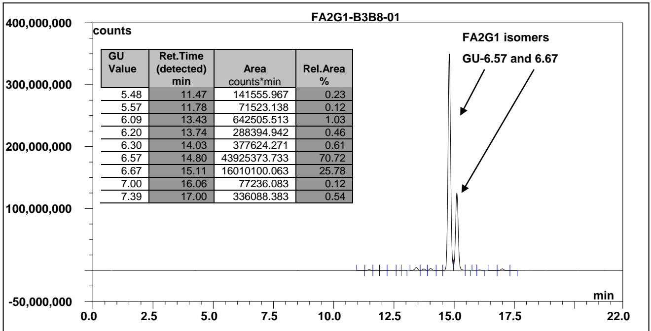
Figure 3: BEH Glycan column chromatogram of 2AB labelled FA2G1 glycan (CN-FA2G1-10U, Batch B3B8-01).
