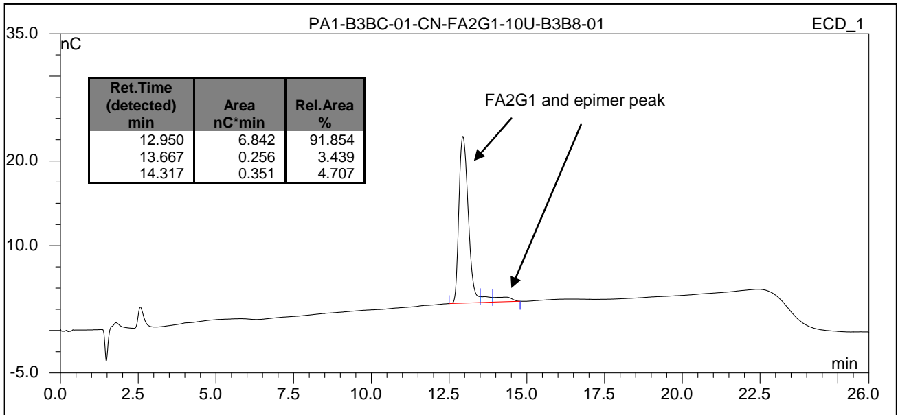
Figure 1: HPAE-PAD HPLC Profile of FA2G1 (CN-FA2G1-10U, Batch B3B8-01).
