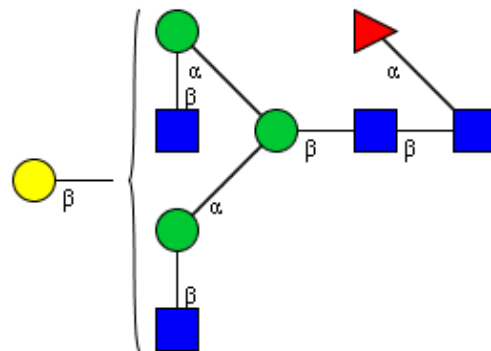
CFG Notation
