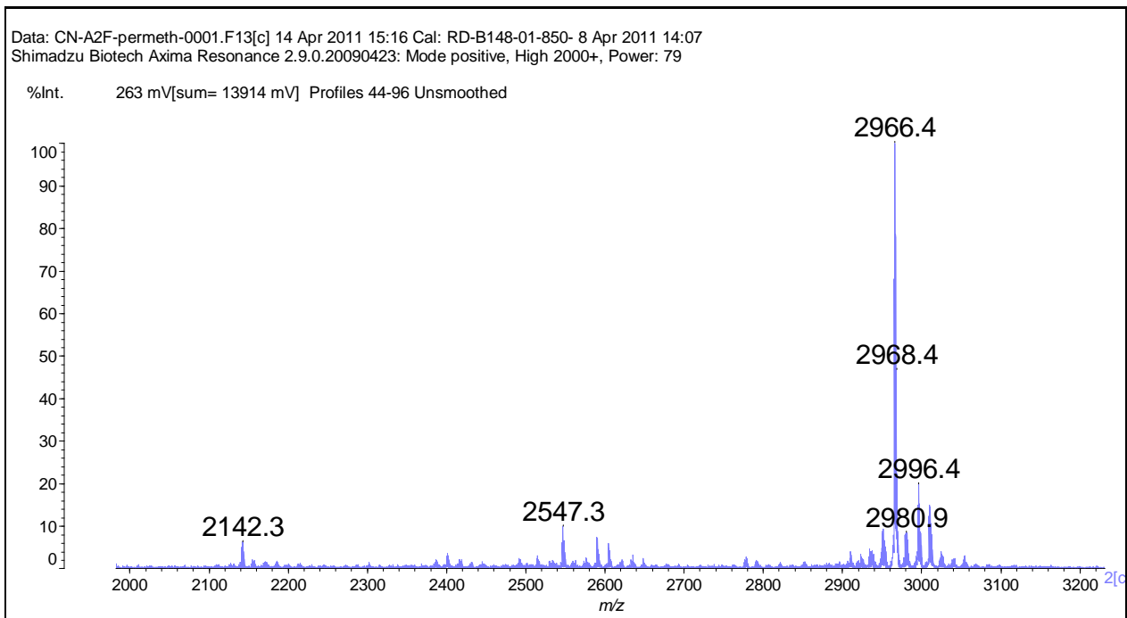
Figure 4: Positive ion mass spectrum of permethylated A2F glycan (CN-A2F-20U, Batch B132-01). Theoretical mass 2966.5 Da [M+Na]^+ .
