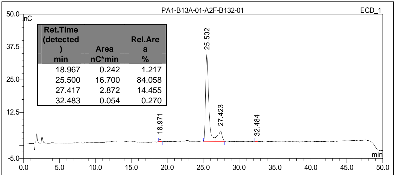
Figure 1 : HPAE-PAD HPLC Profile of A2F (CN-A2F-20U, Batch B132-01).
