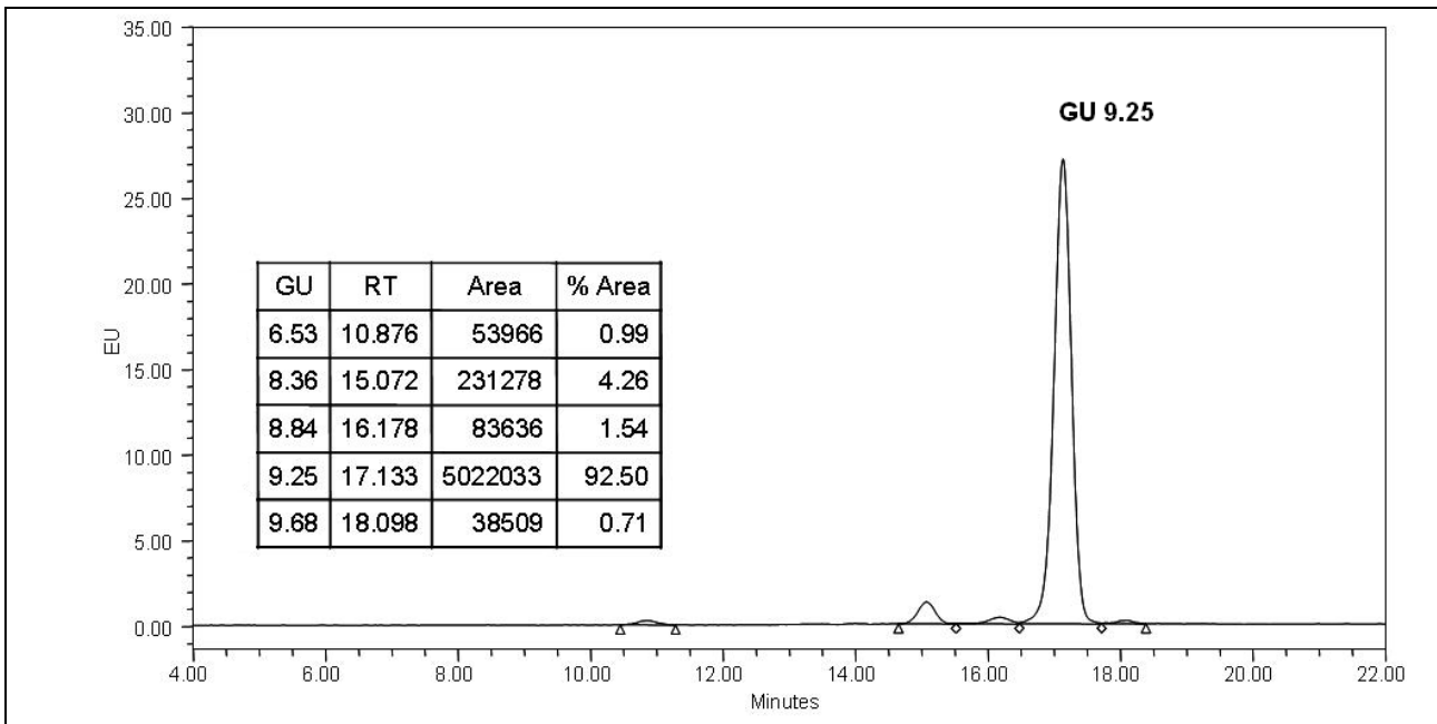
Figure 3: LudgerSepN2 chromatogram of 2AB labelled A2F glycan (CN-A2F-20U, Batch B132-01).
