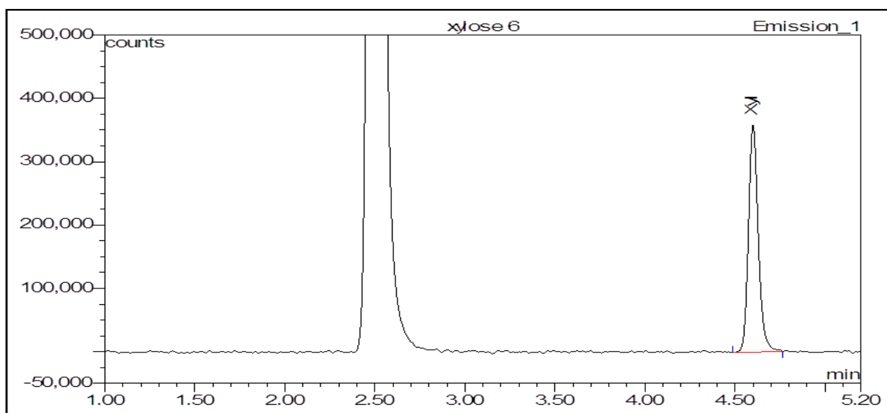
Figure 1: Ludger Sep-UR2 column profile of CM-XYL-100 -2AA labelled. The peak between 2-3 minutes is free dye. Sample run 24 TH JUNE-2015.
