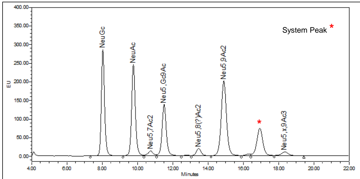
Figure 1: LudgerSep UR2 HPLC profile of DMB labeled Sialic acid Reference Panel
