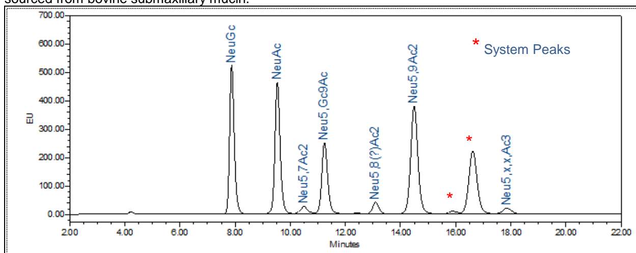
Figure 1: LudgerSep R1 HPLC profile of DMB labeled Sialic acid Reference Panel (Cat. #: CM-SRP-01, Batch B69E-01).
