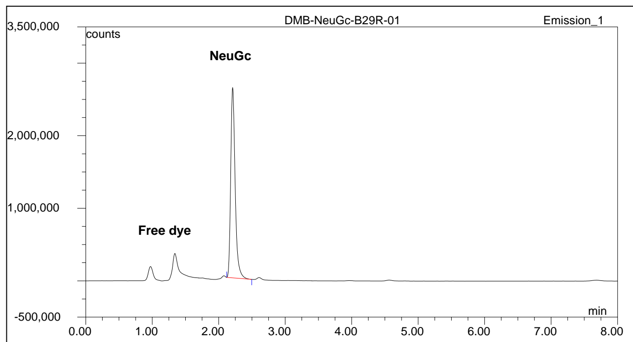
Figure 1: LudgerSep-uR2 HPLC profile of 1,2-diamino-4,5-methylenedioxybenzene.2HCl (DMB) labeled NeuGc standard (Cat. #: CM-NEUGC-01, Batch B29R-01).
