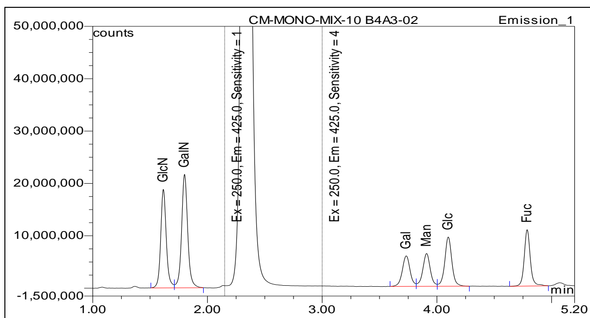
Figure 1: LudgerSep-uR2 HPLC profile of 2-aminobenzoic acid (2-AA) labeled mono-mix. (Cat. #: CM-MONO-MIX-10, Batch B4A3-02). The peak between 2 to 3 min is free dye.
