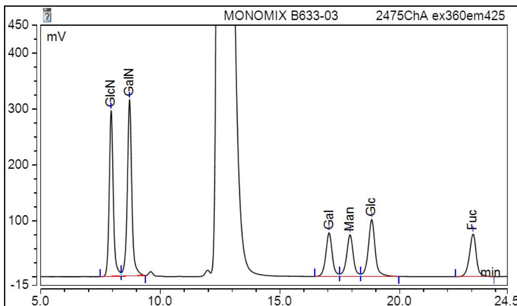
Figure 1: LudgerSep-R2 HPLC profile of 2-aminobenzoic acid (2-AA) labeled mono-mix. (Cat. #: CM-MONO-MIX-10, Batch B633-03). The peak between 12 to 14 min is free dye.
