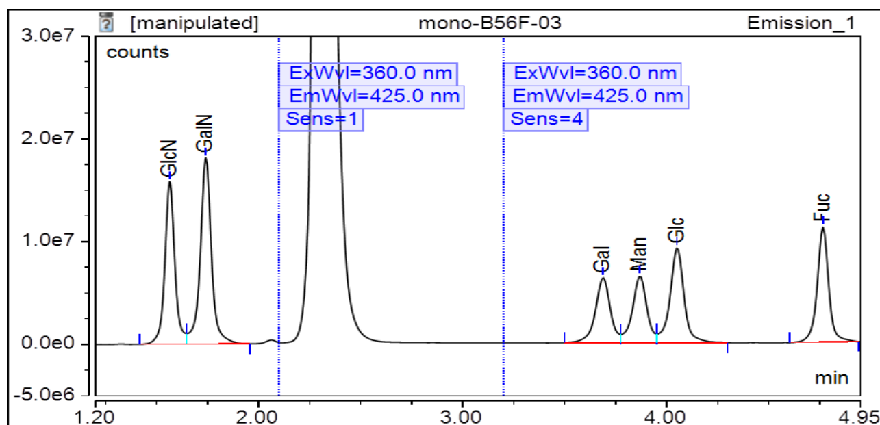
Figure 1: LudgerSep-uR2 HPLC profile of 2-aminobenzoic acid (2-AA) labeled mono-mix.
