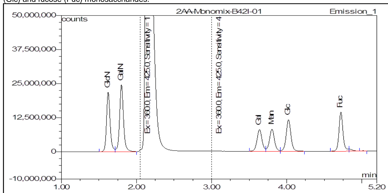
Figure 1: LudgerSep-uR2 HPLC profile of 2-aminobenzoic acid (2-AA) labeled mono-mix.
