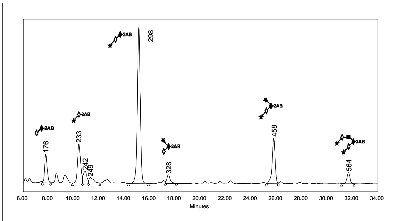
Figure 1: LudgerSep-N2 HPLC Profile of 2AB Labelled Fetuin O-Glycans (Cat. No. CLIBO-FETUIN-01, Batch No. B23D-04).
