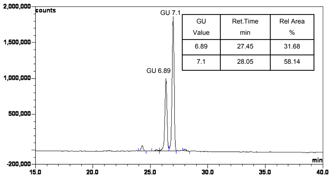
Figure 1: BEH uHPLC profile of APTS Labeled FA2G1 Glycan (Cat. #: CAPTS-FA2G1-01, Batch # B283-02).
