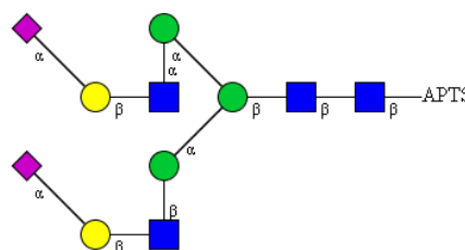
CFG Notation
