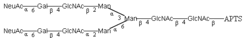
Text Notation
