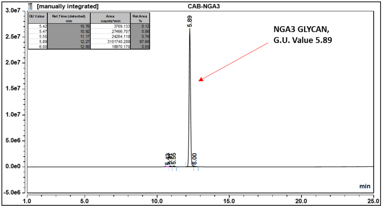
Figure 1: HILIC HPLC profile of 2AB labelled NGA3 glycan (see method conditions below) (Cat. #: CAB-NGA3-01, Batch B381-05).
