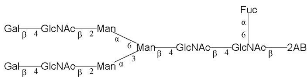
Text Notation
