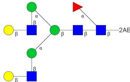
CFG Notation
