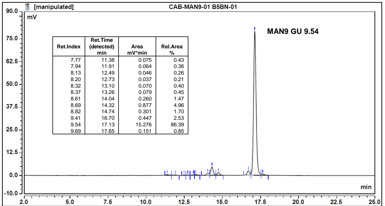
Figure 1: HILIC HPLC profile of 2AB labelled MAN9 glycan (see method conditions below)
