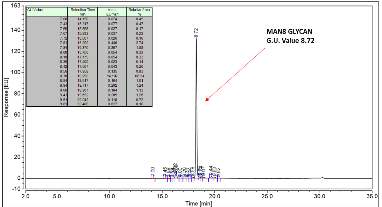
Figure 1: HILIC HPLC profile of 2AB labelled MAN8 glycan (see method conditions below)
