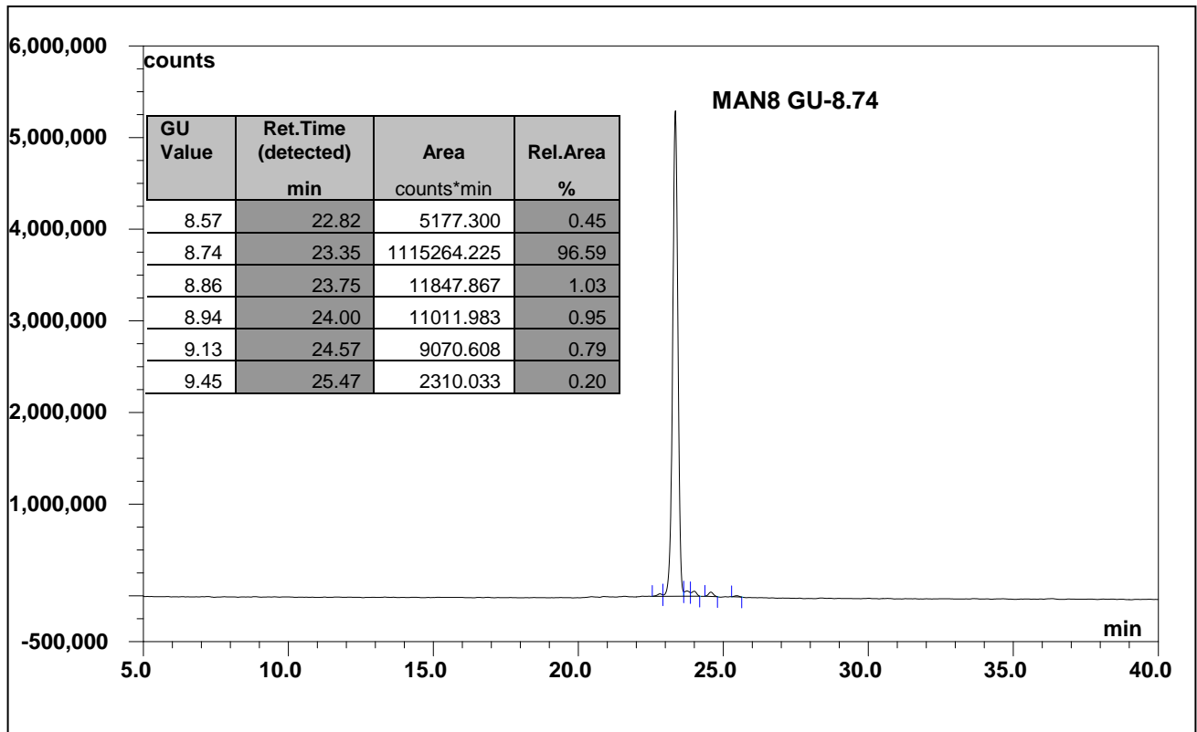
Figure 1: HILIC HPLC profile of 2AB labelled MAN8 glycan (see method conditions below) (Cat. #: CAB-MAN8-01, Batch B325-08).
