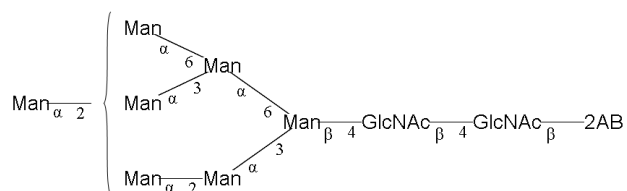
Text Notation
