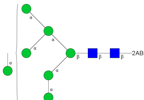
CFG Notation
