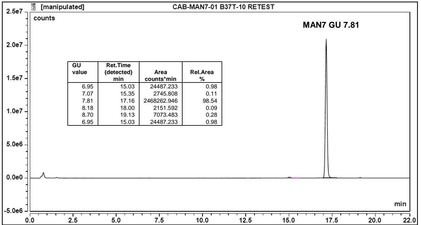
Figure 1: HILIC HPLC profile of 2AB labelled MAN7 glycan (see method conditions below)
